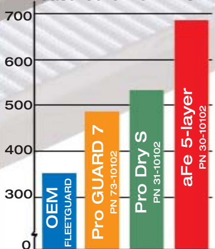
CFM Graph, Dodge Cummins Measured @ 1.5" H2O
