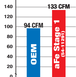
P/N 54-11291
