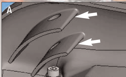
Patent-pending internal air vanes (←) smooth and direct airflow for minimal pressure loss and maximum CFM gains.
