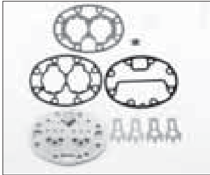
Valve Plate (Canted, Side Bank w/HGBP) Order Part #: P-17-44104-00 (Replaces Carrier #: 17-44104-00)
