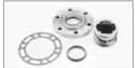
Seal, Shaft (05D) Order Part #: P-17-44135-00 (Replaces Carrier #: 17-44135-00)
