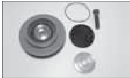
Pulley, Idler Order Part #: P-50-01152-20SV (Replaces Carrier #: 50-01152-20SV)
