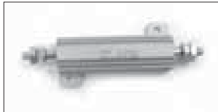
Resistor (50W) Order Part #: P-22-01427-00 (Replaces Carrier #: 22-01427-00)
