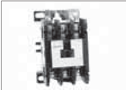
Contactor, Compressor (40A) Order Part #: P-10-00304-33 (Replaces Carrier #: 10-00304-33)
