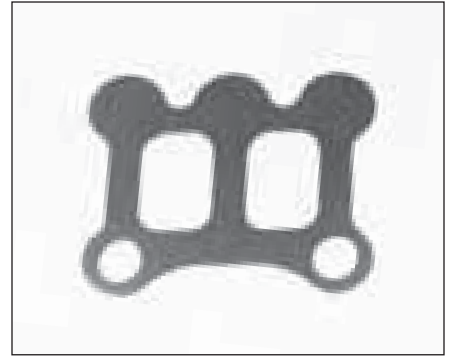
Valve, Discharge Order Part #: P-17-40086-00 (Replaces Carrier #: 17-40086-00)
