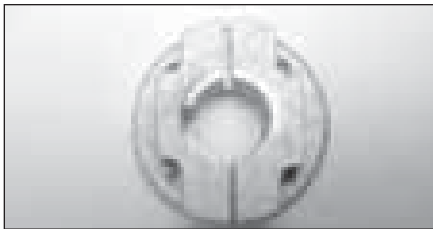
Adapter, Condenser Fan Order Part #: P-48-60001-00 (Replaces Carrier #: 48-60001-00)
