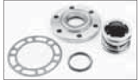
Seal, Shaft (05G) Order Part #: P-17-44145-00 (Replaces Carrier #: 17-44145-00)
