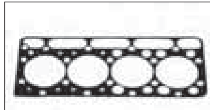
Gasket, Head (134DI) Order Part #: P-25-38529-01-B (Replaces Carrier #: 25-38529-01)
